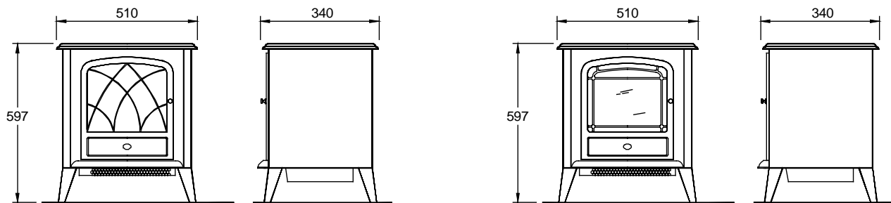
Ritz Stove
