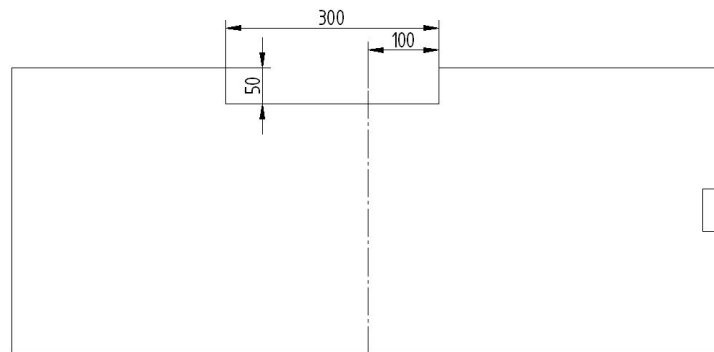
DROLET DIESEL S/S INNER SHIELD WETBACK CUTOUT
