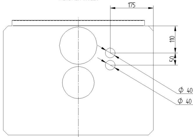
DROLET DIESEL REAR HEATSHEILD WETBACK HOLES
